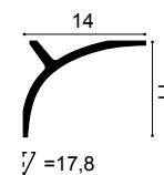
① C991 Purotouch® 200 x 11 x 14 cm Designed by Ulf Moritz
